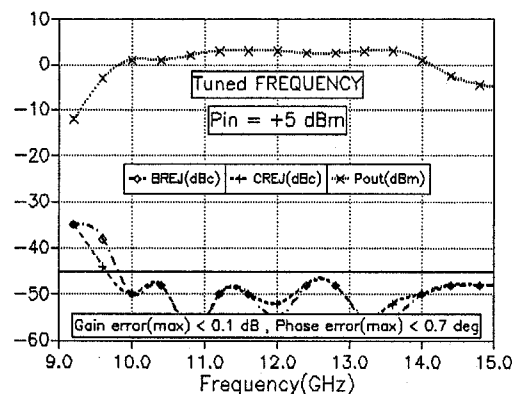
Figure 7 Measured output power, carrier and side band rejection function of frequency
